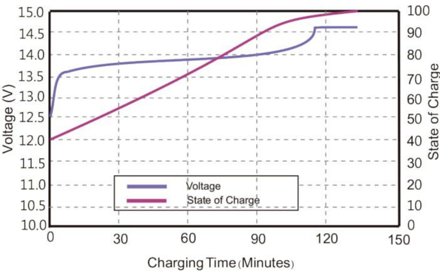
State of Charge Curve @0.5C 25
