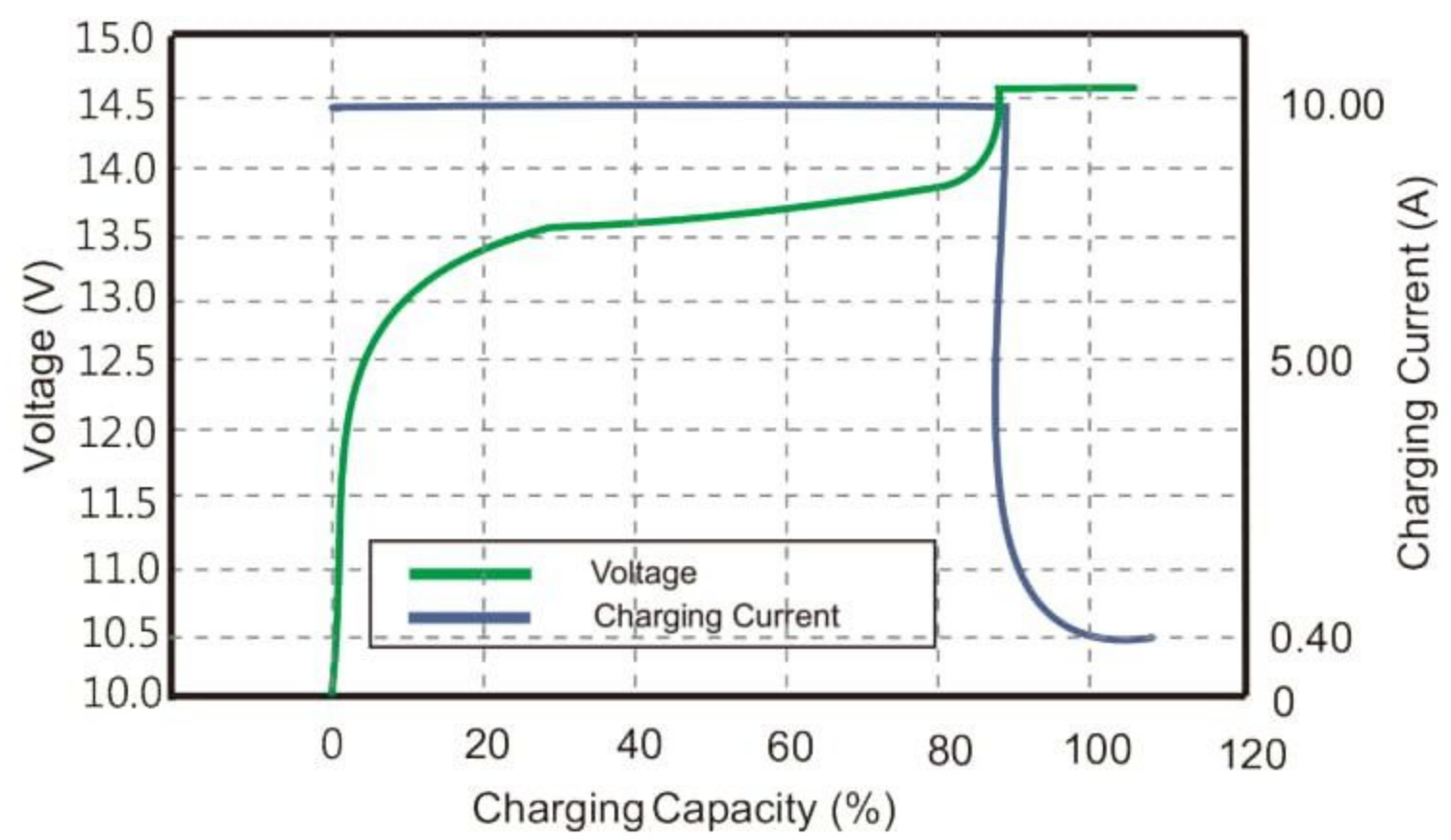
Charging Characteristics @0.5C 25
